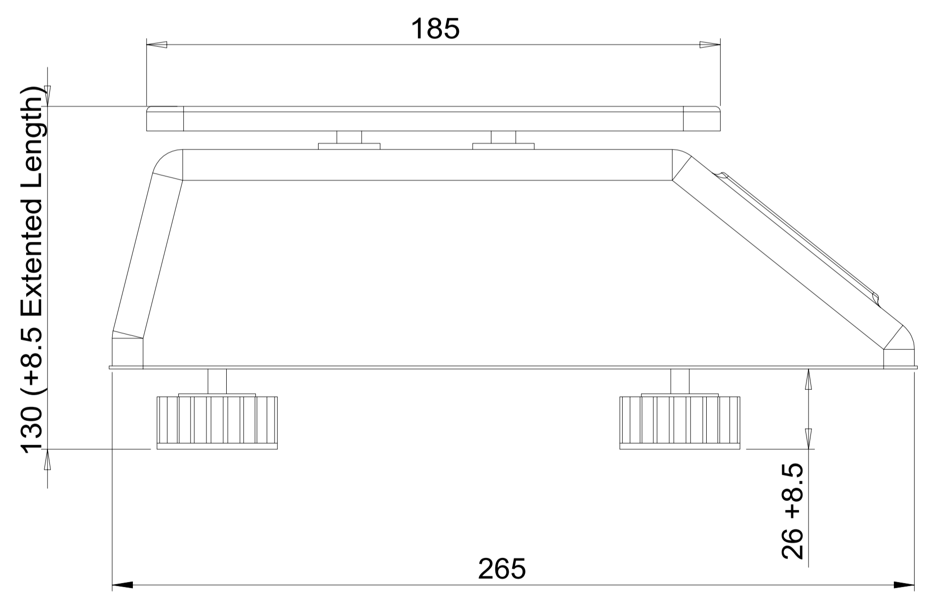
SIDE VIEW
