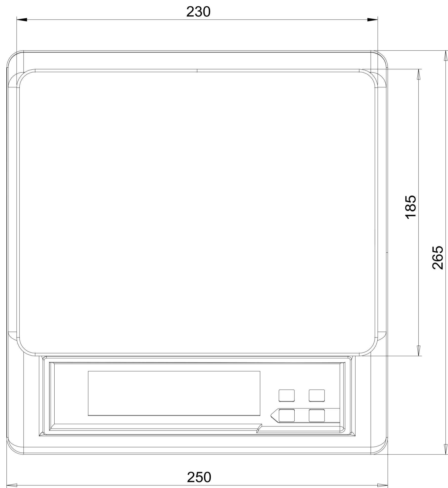
TOP VIEW
